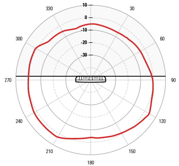
ELEVATION 5 GHZ
